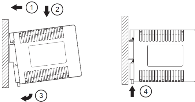
Fig. 2.1 Mounting
