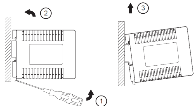
Fig. 2.2 Dismounting
