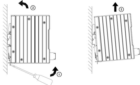
Fig. 2.2 Dismounting
