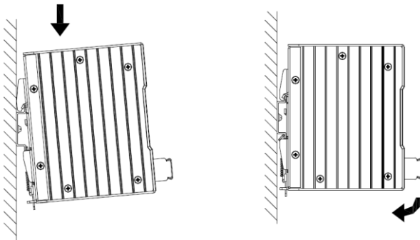
Fig. 2.1 Mounting
